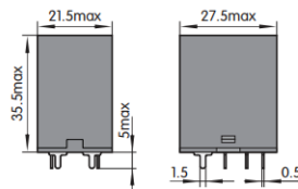
Outline drawing (lateral flange type)
