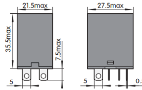
Outline drawing (PCB type)
