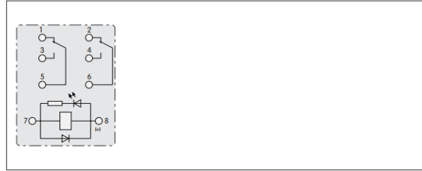
PCB opening drawing (2Z)
