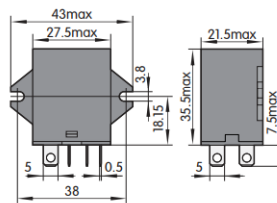
Outline drawing (top flange type)
