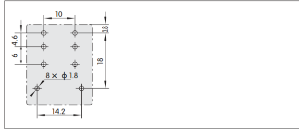
Outline drawing (plug-in type)
