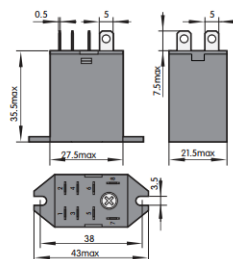
Outline drawing (top flange type)
