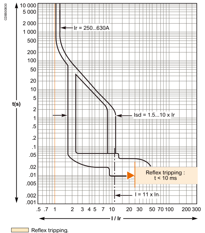
ETS2.3 630 A
