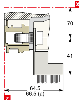
DB115459 CVS100 to 250
