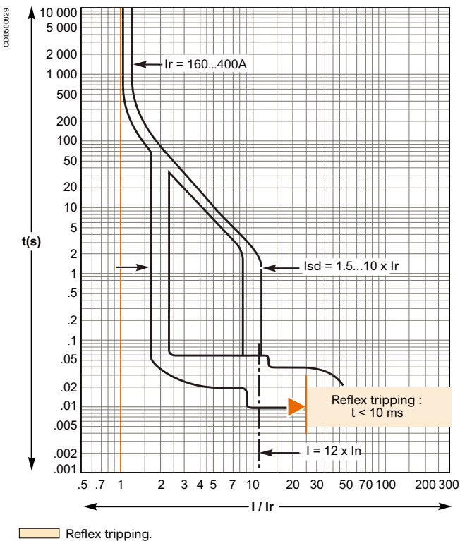
ETS2.3 400 A
