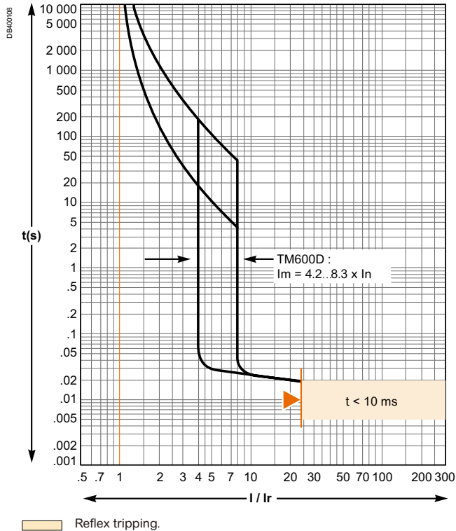
TM600D
