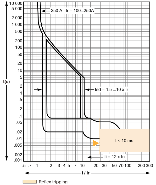
ETS2.2 250 A
