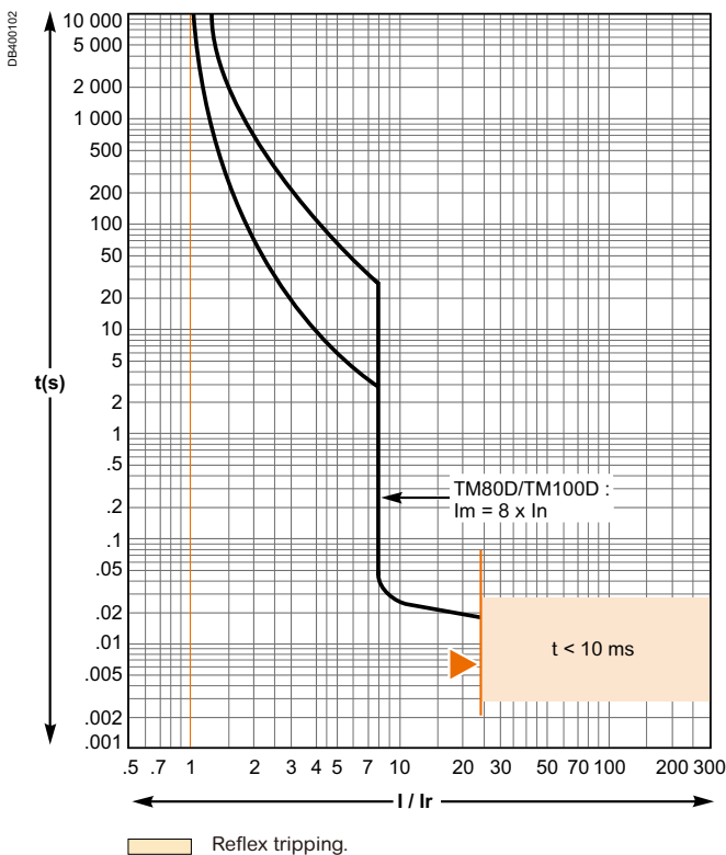
TM80D/100D
