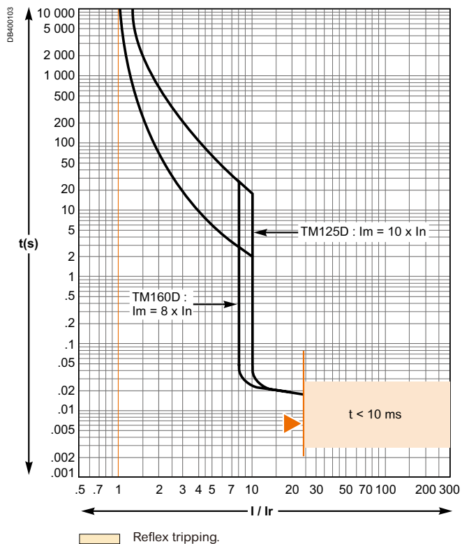
TM125D/160D
