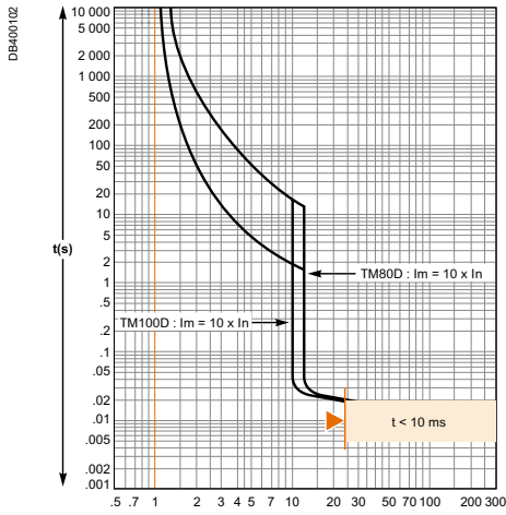
Reflex tripping.
