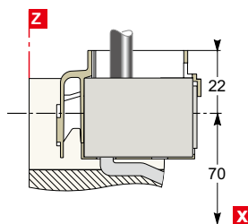
DB115454 CVS400/630
