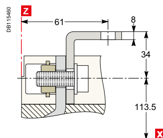
DB115460 CVS400/630
