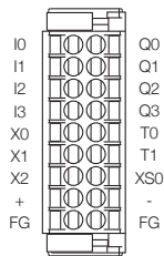
FX5-SF-MU4T5
