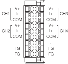
FX5-4AD
