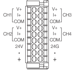
FX5-4DA
