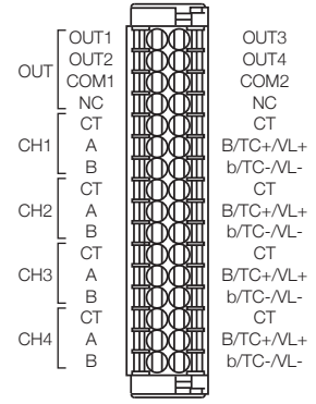
FX5-4LC
