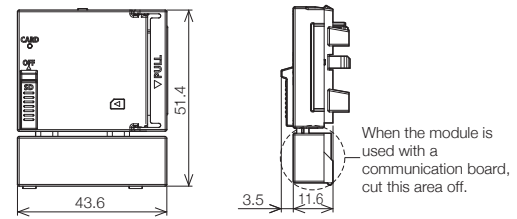
FX5-SDCD
