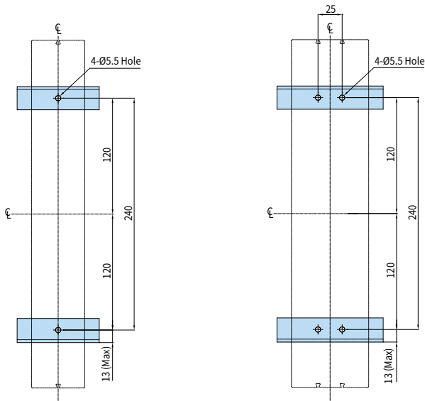
Mounting Drawing
