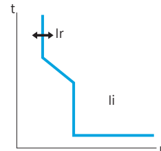
Characteristics Curve (I - t Curve)
