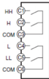
Relay Outputs <C2>
