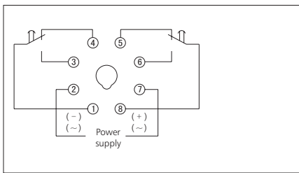
NJS1-ZZ Wiring diagram
