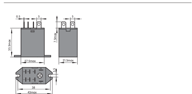
Outline drawing (top flange type)
