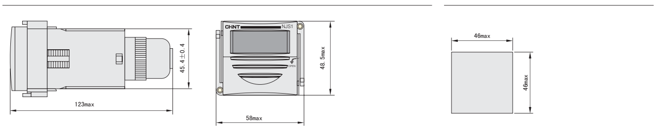
Opening size
