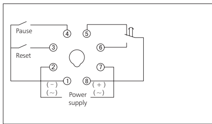
NJS1-11 Wiring diagram
