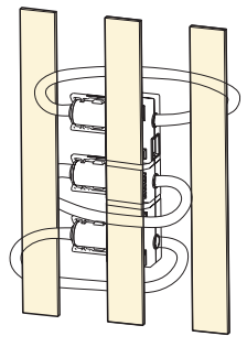
Figure 7 Transformer mounting type 2
