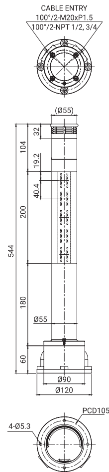
·QST50BT-Ex-5-DC/AC
