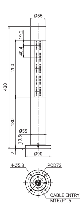
·QST50T-Ex-5-DC/AC
