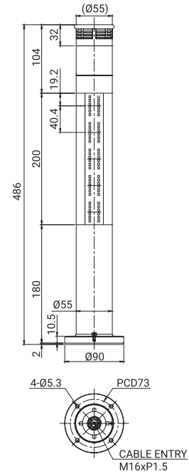
·QST50BT-Ex-5-DC/AC
