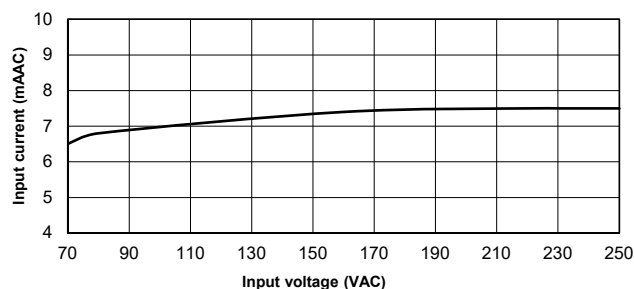
RL..A.: AC input current vs. input voltage
