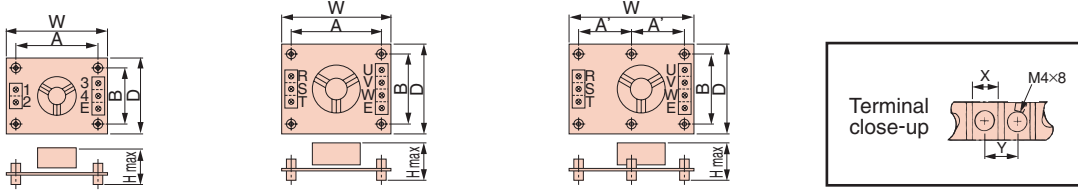
Figure 1 (Single-Phase) Figure 2 (Three-Phase) Figure 3 (Three-Phase)
